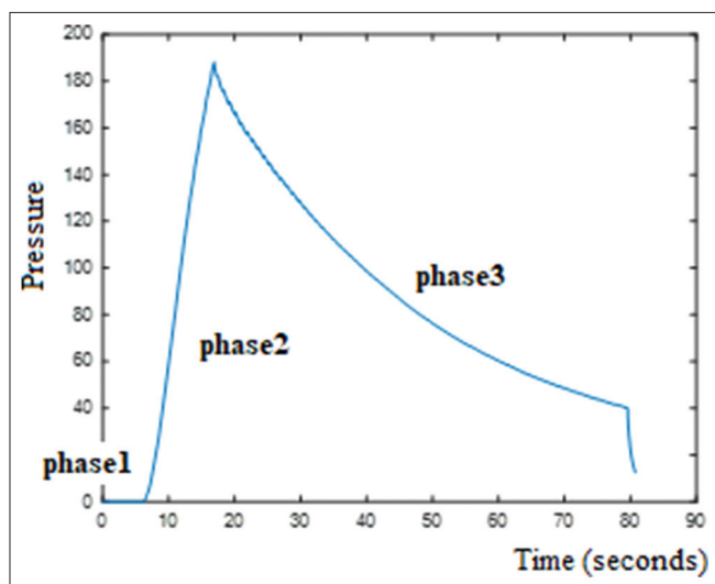
Figure 5: Pressure phases
