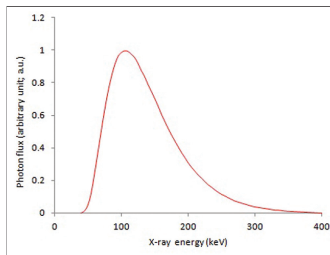
Figure 1: X-ray spectrum of European Synchrotron Radiation Facility ID17 medical beam line, with a 16-mm-thick aluminum filter
