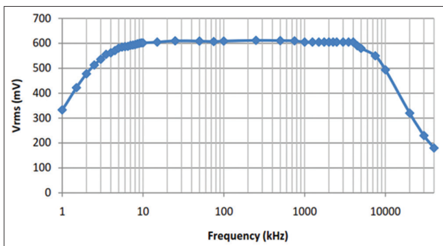
Figure 5: V_{rms} versus frequency was produced by AD9850
