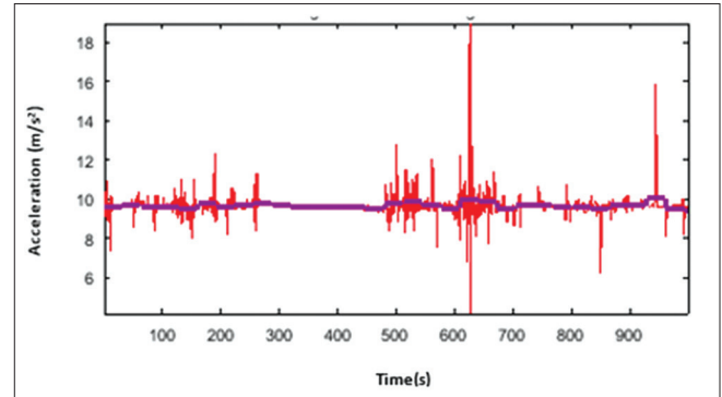
Figure 10: The original signal (in red) and the filtered signal user
