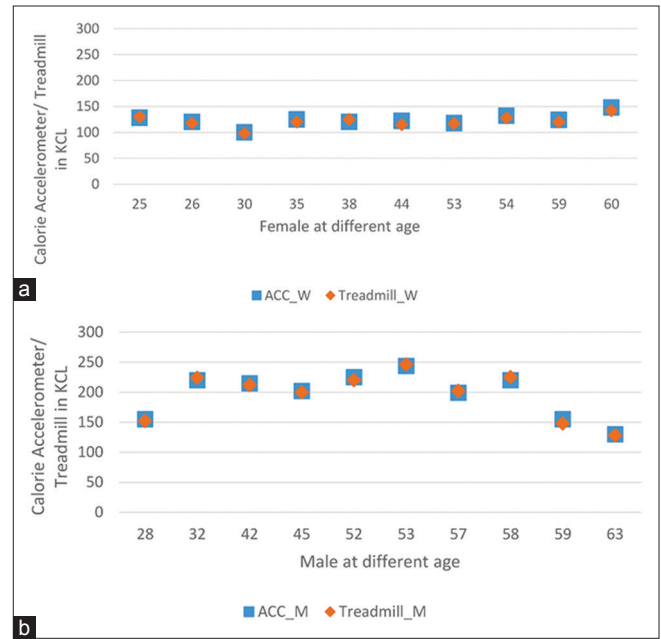
Figure 16: The calorie consumption comparison between the accelerometer and the treadmill for (a) female and (b) male
