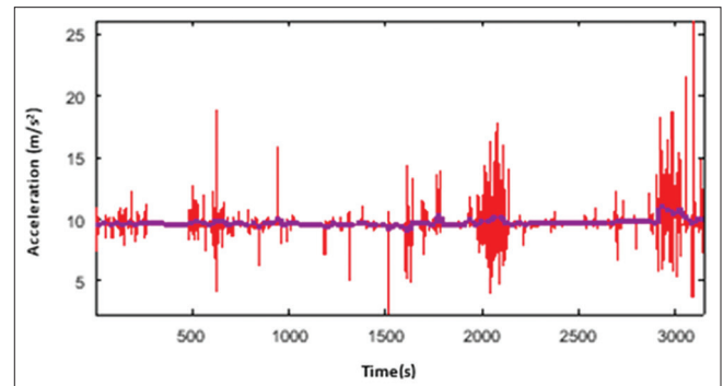
Figure 11: The original signal (in red) and the filtered signal (in purple) from the running activity of a single user
