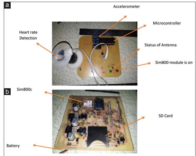
Figure 2: (a) Kit's front view, (b) kit's back view
