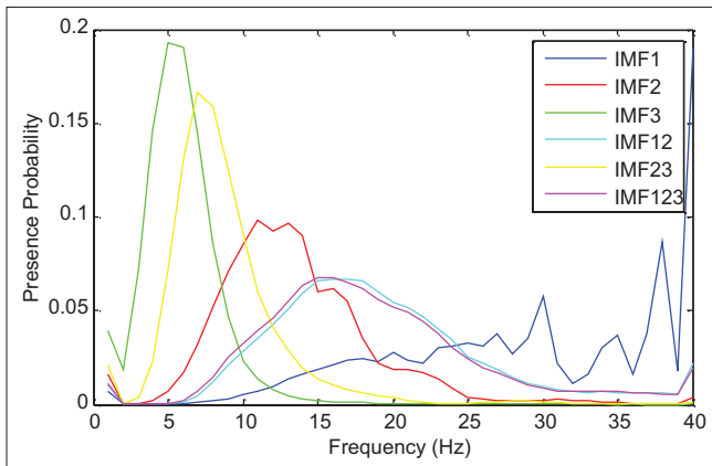
Figure 3: The instantaneous frequency histogram for six-intrinsic mode function-combination conditions
