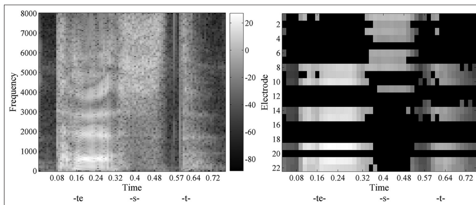
Figure 6: The spectrogram of the original acoustic signal (the word “test”) at the microphone input of the sound processor (left). And the corresponding electrodiagram using results obtained from undecimated wavelet strategy (right). The decomposition was done by N-of-M strategy (8 channels out of 22). The colormap shows the intensity
